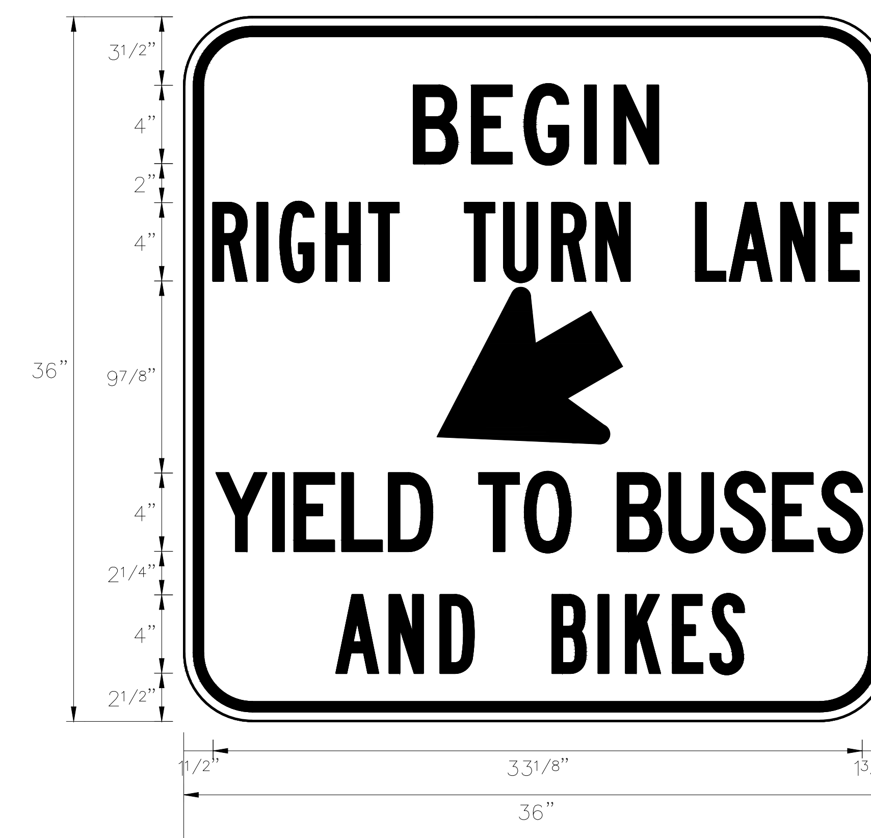
SP-4 SIGN DETAIL NOT TO SCALE
