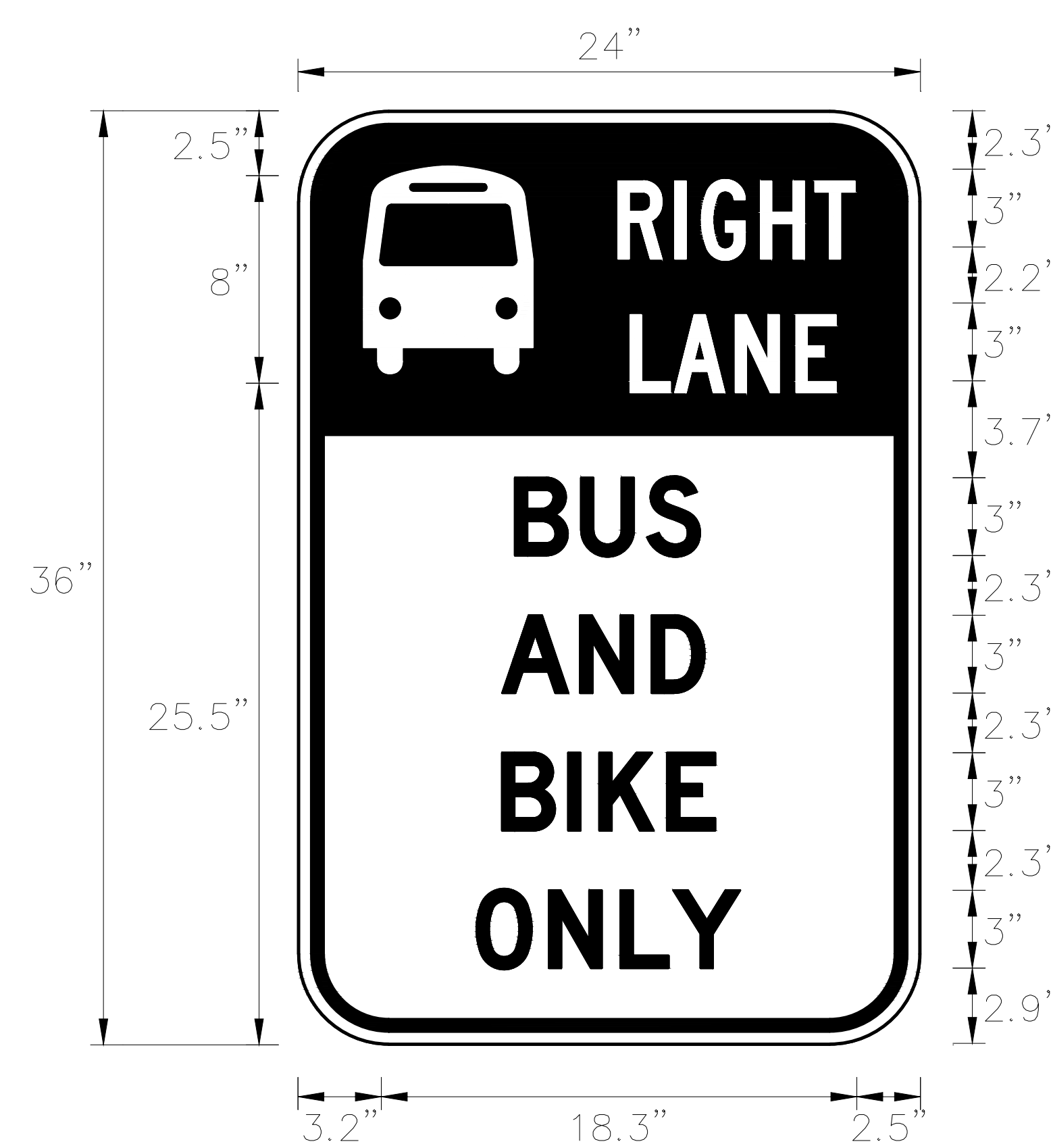
SP-2 SIGN DETAIL NOT TO SCALE
